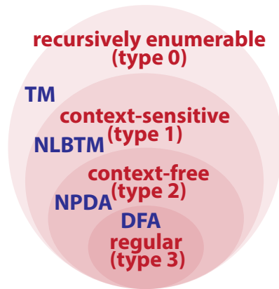
Venn diagram of Chomsky hierarchy and automata models
