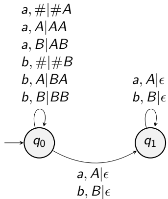
deterministic and non-deterministic pushdown automata (NPDA/PDA)
